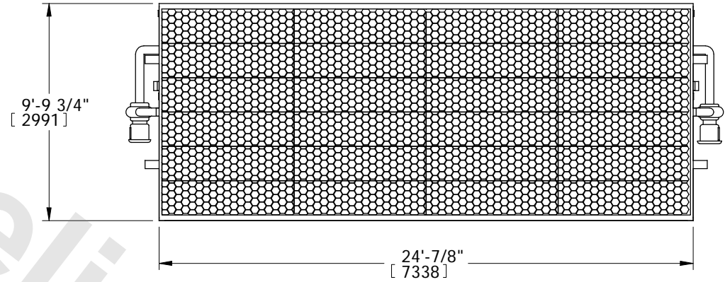
FACE 1 PLAN VIEW
